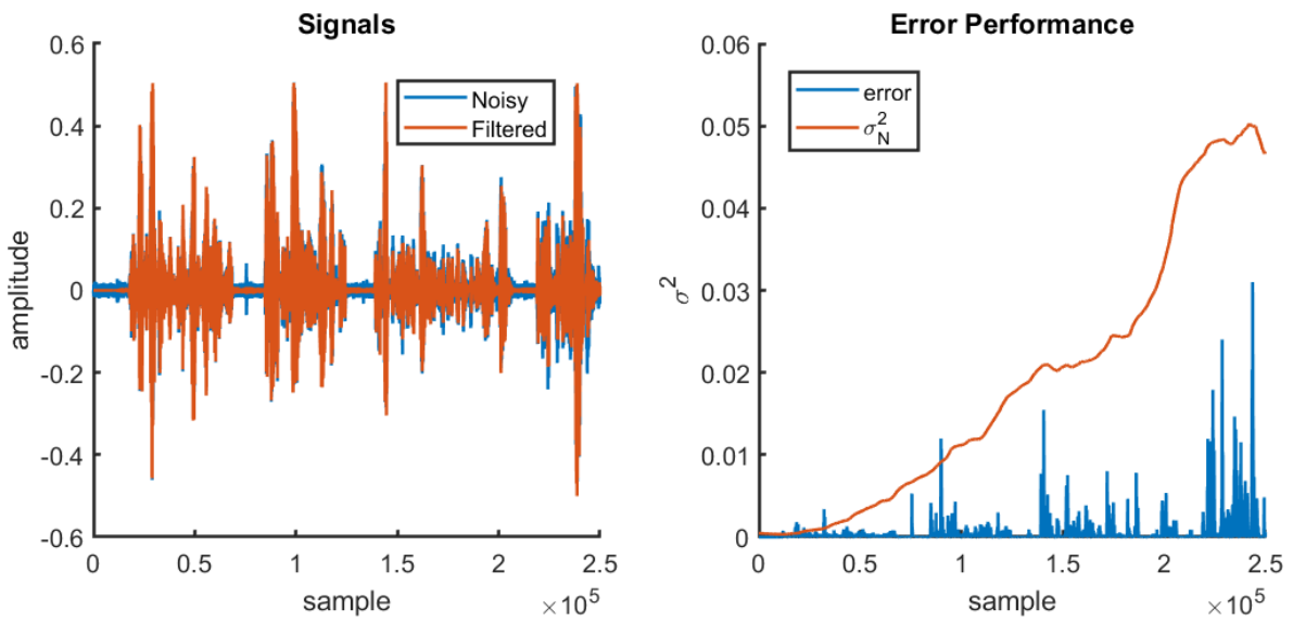
Fig. 6: Results of the Minimal Statistics based approach using K=\text{Inf} .
